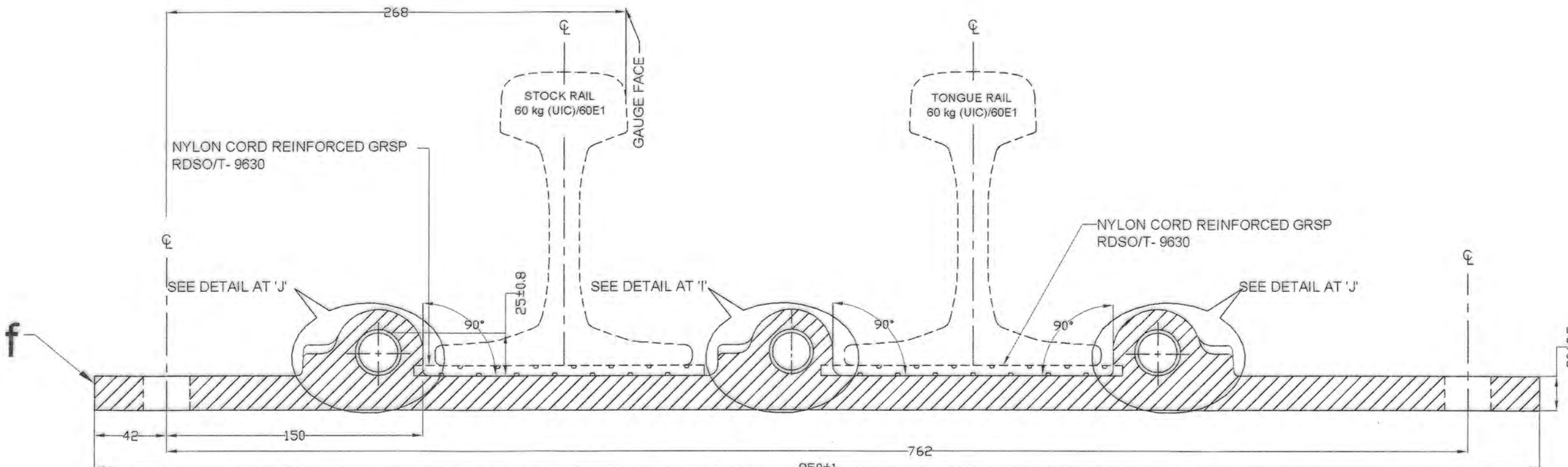
SECTIONAL ELEVATION ON GH
