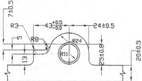
DETAIL 'I'
